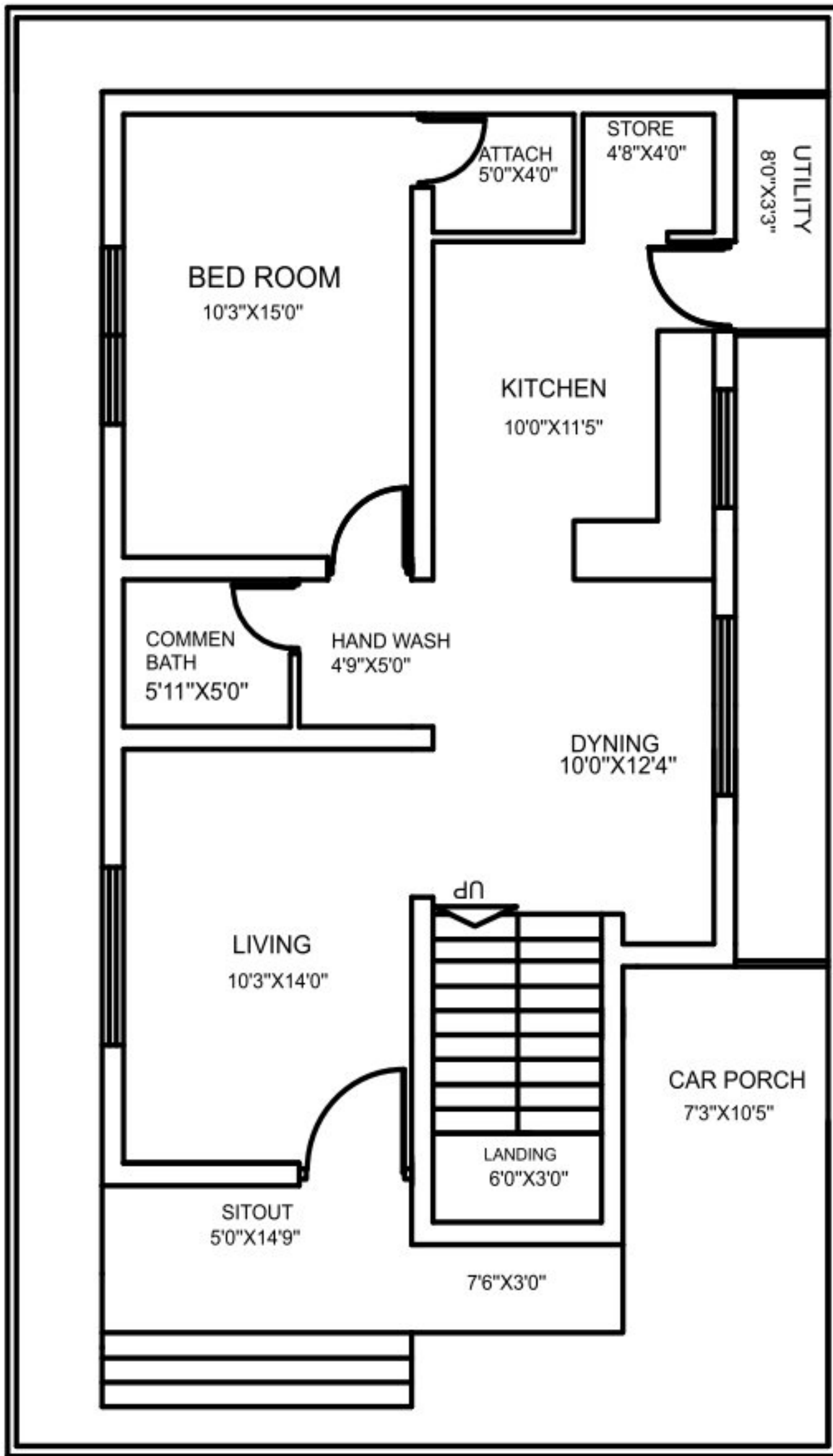
GROUND FLOOR
