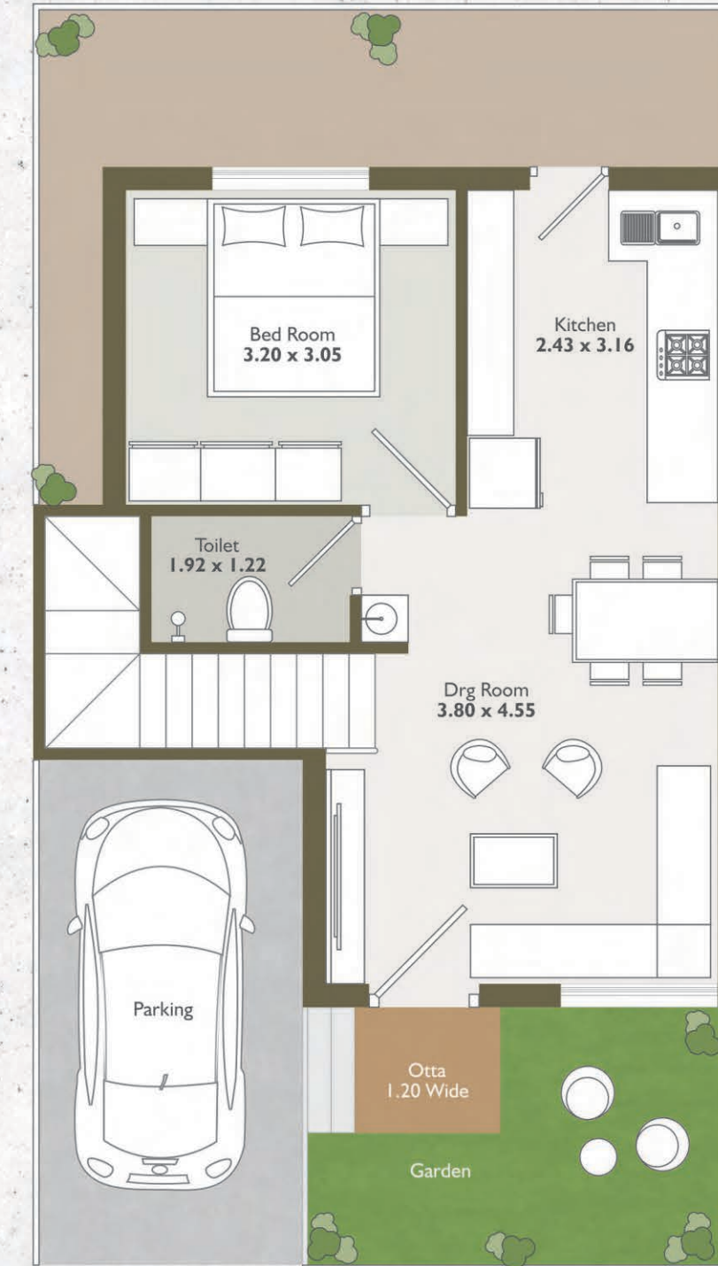
Ground Floor
