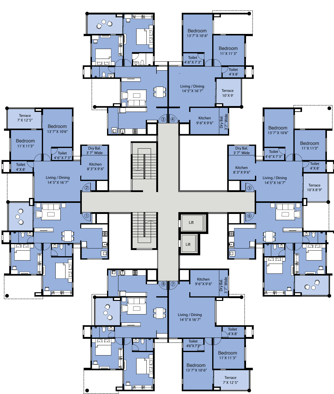
2 BHK LUXURY - A , B , C , D BUILDING ODD FLOOR PLAN
