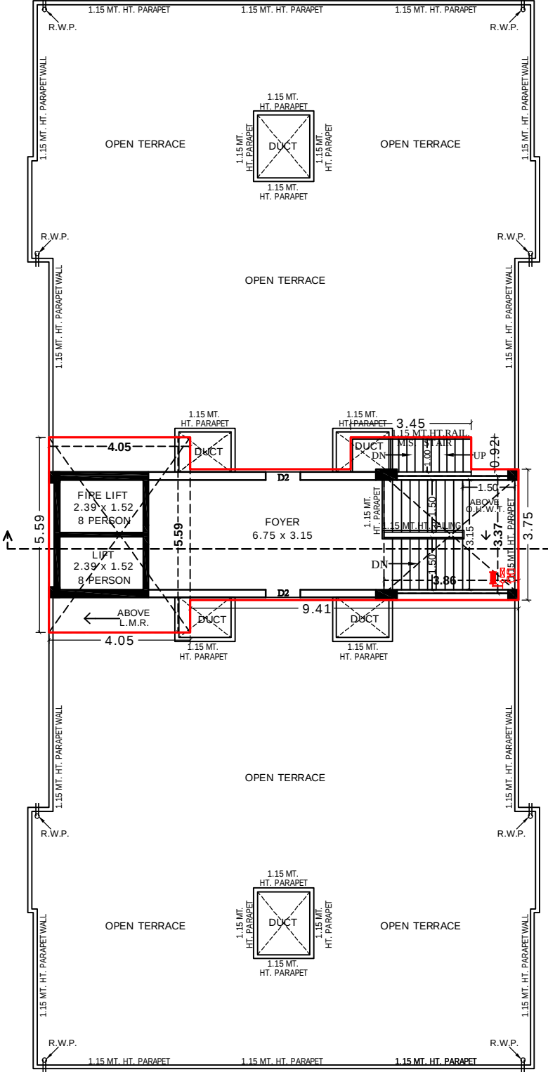
STAIR CABIN , L.M.R. & OPEN TERRACE PLAN
