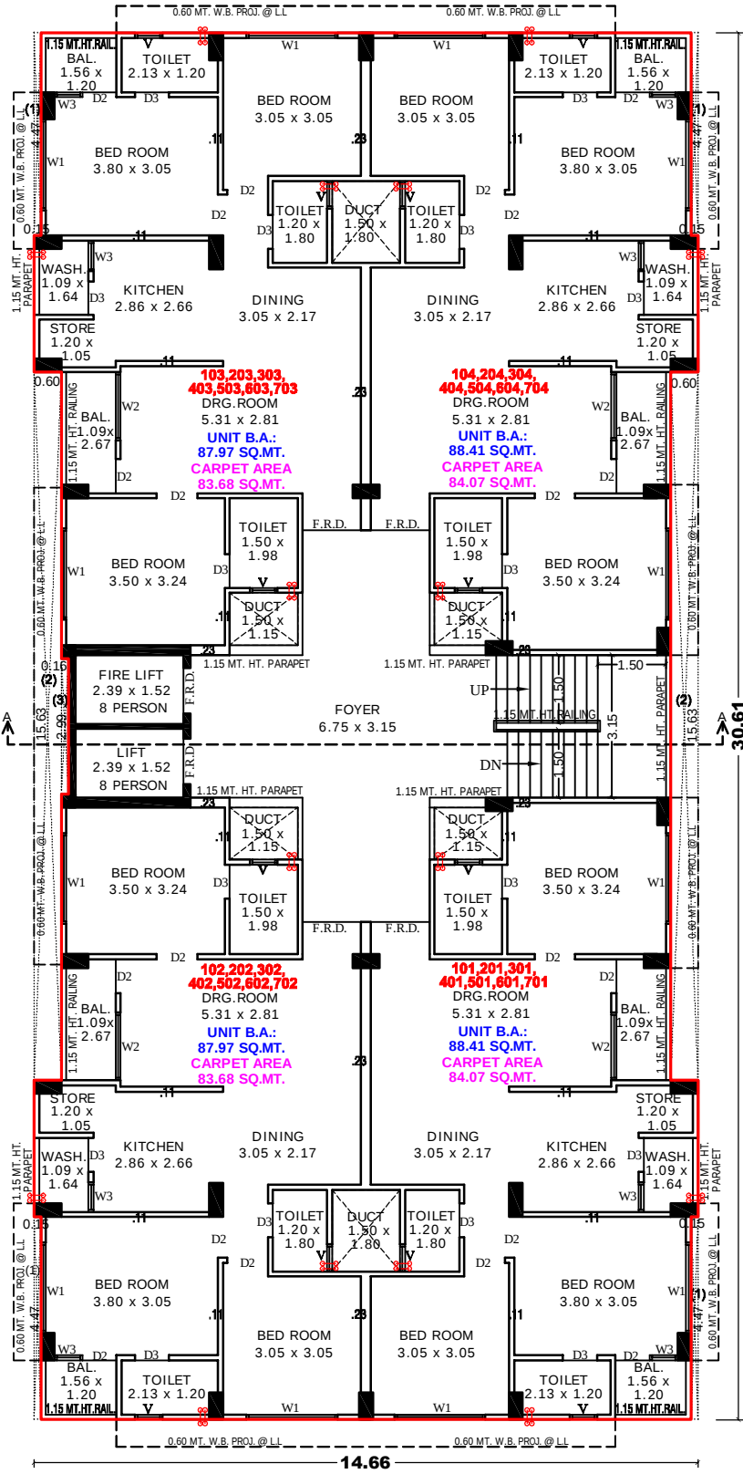
1ST .FL. TO 7TH. FL. PLAN
