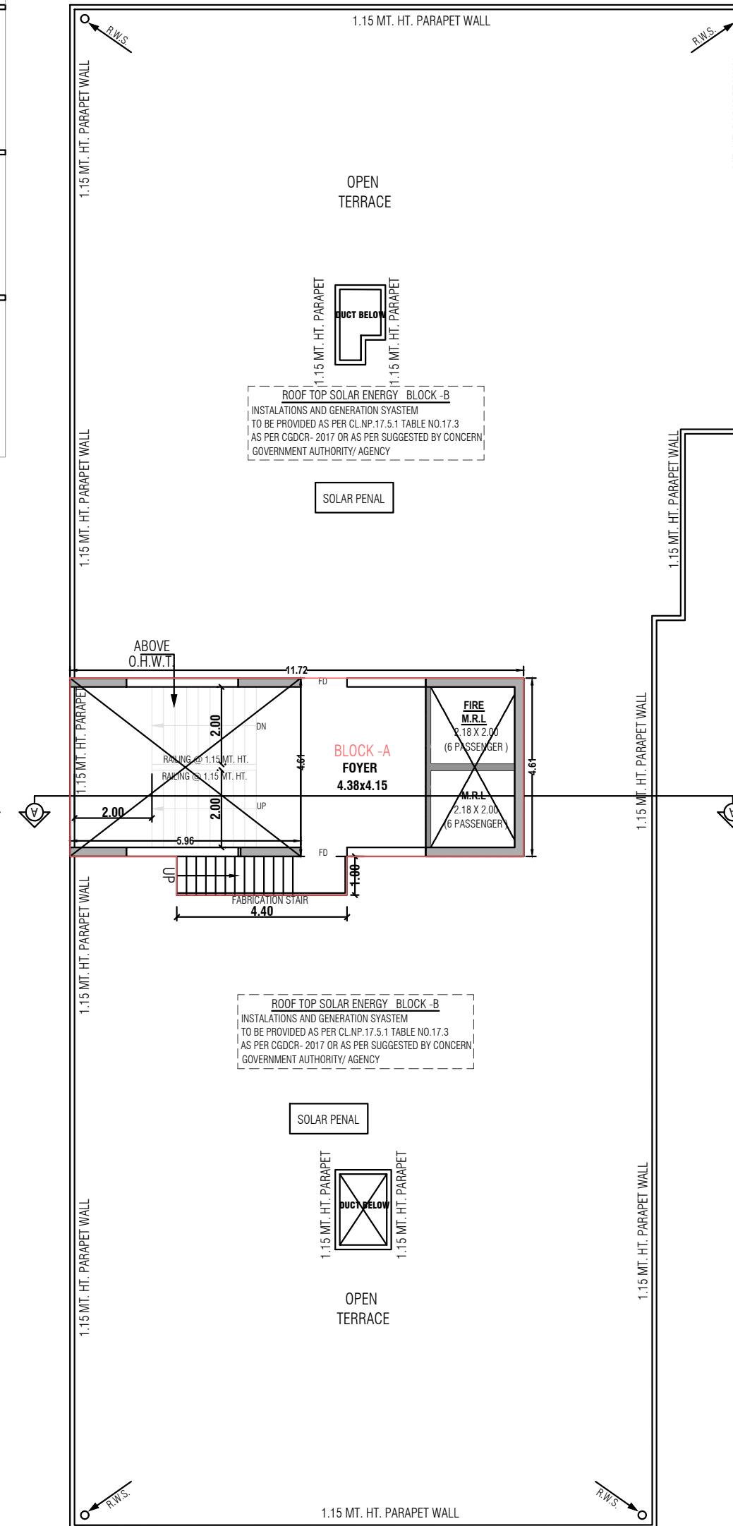
OPEN TERRACE & STAIR CABIN PLAN
