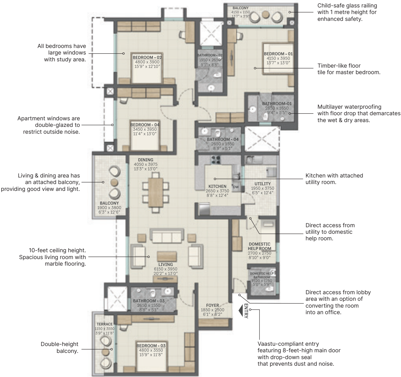
Key plan
