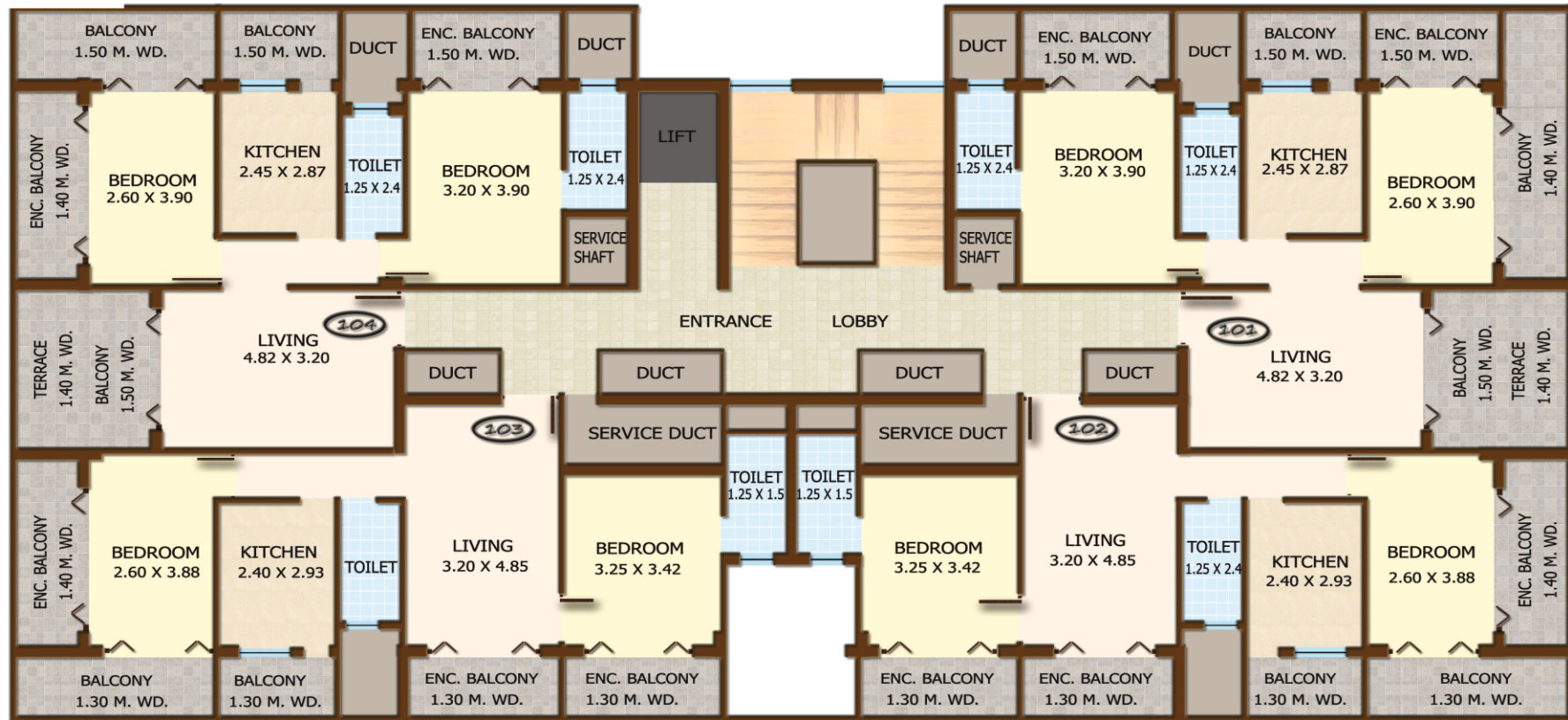
TYPICAL UPPER GROUND/ SECOND FLOOR PLAN
